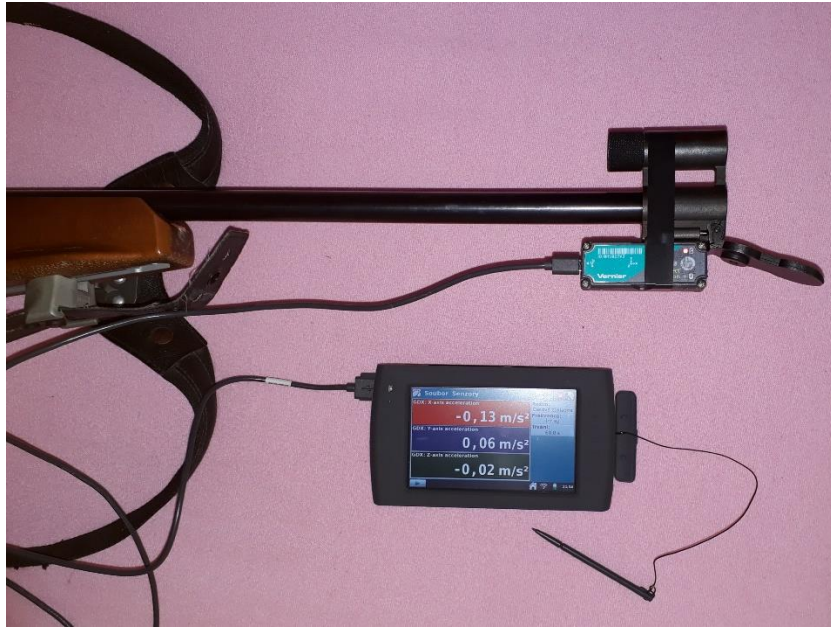
Figure 3. Rifle with accelerometers connected through light weight cable with digital device.
