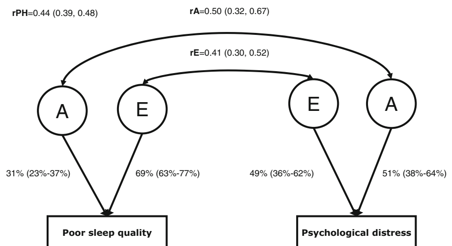
FIGURE 1 Bivariate model poor sleep quality and psychological distress. A, additive genetic influences; E, non-shared environmental influences. r_A , additive genetic correlation; r_E , non-shared environmental correlation; r_{PH} , phenotypic correlation. r_{PH} , r_A , and r_E were statistically significant ( p < 0.001 )
