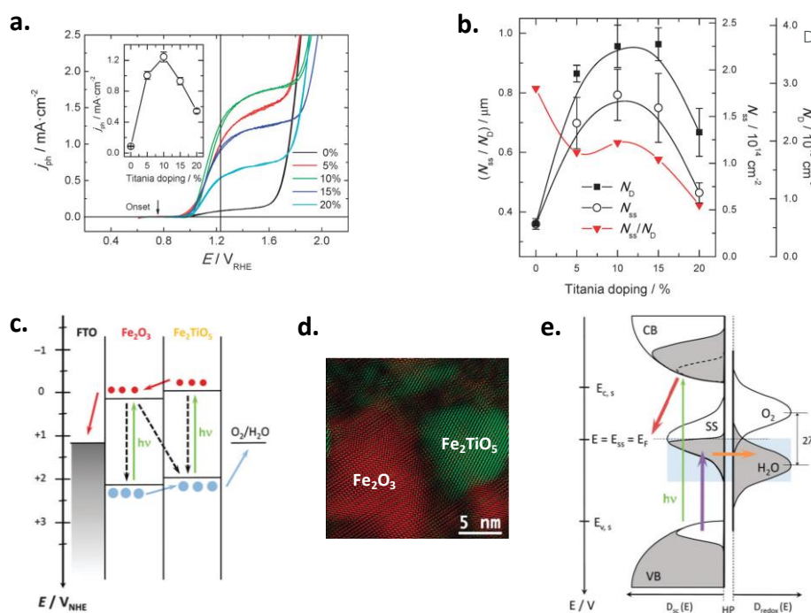
Fig. 4 (a) Voltammetric measurements for hematite/titania electrodes under illumination with different titania doping; the vertical line depicts the thermodynamic potential value of the oxygen evolution reaction ( 1.23 V_{\text{RHE}} ); the inset shows the photocurrent density values at 1.23 V_{\text{RHE}} as a function of titania doping. (b) Donor density ( N_D ), total surface state density ( N_{\text{SS}} ) and their ratio ( N_{\text{SS}}/N_D ) as a function of titania doping; N_D was estimated from the slopes of the respective Mott-Schottky plots in the dark; N_{\text{SS}} was obtained from integration of the density of surface states profiles, estimated from impedance measurements under illumination. (c) Thermodynamic scheme of the charge generation, transfer and recombination processes at the biased ( 1.23 V_{\text{RHE}} ) hematite/titania electrode under illumination, for intermediate and optimum titania doping values (5-15%). (d) HR-TEM micrograph of the hematite/titania 20% sample, shown as a coloured inverse FFT image highlighting the hematite ( \text{Fe}_2\text{O}_3 , red) and pseudo-brookite ( \text{Fe}_2\text{TiO}_5 , green) crystallographic phases. (e) Kinetic scheme of the charge generation and transfer processes at the biased ( 1.23 V_{\text{RHE}} ) hematite/titania-electrolyte interface under illumination, for the optimum titania doping values (10-15%). Reprinted with permission from Ref. 91. Copyright 2015 The Royal Society of Chemistry.
