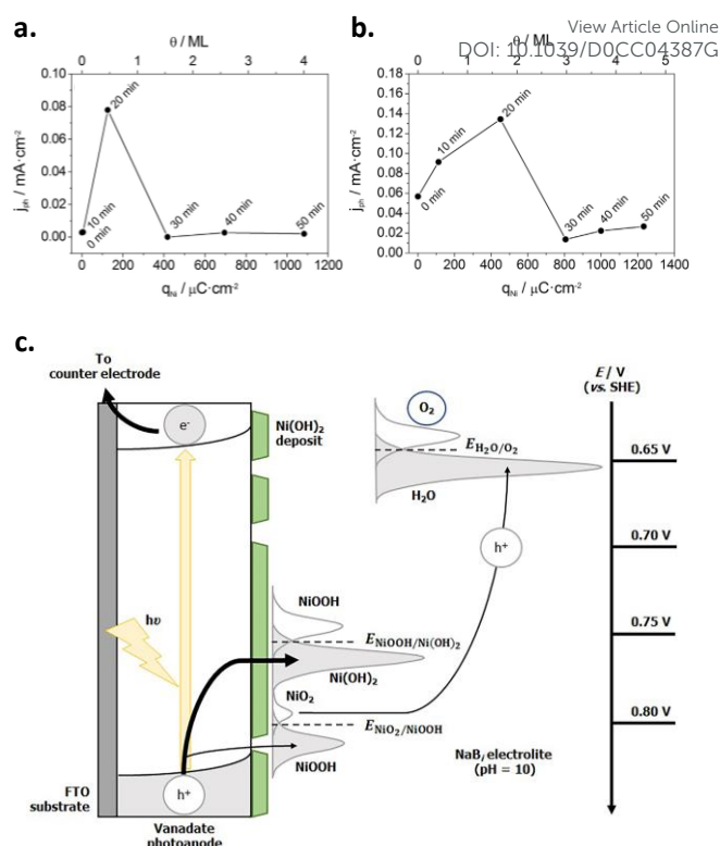
Fig. 7 (a) Photocurrent density for the oxygen evolution reaction (OER) at -0.5 V for BiVO 4 /Ni(OH) 2 photoanodes, prepared with different deposition times (0–50 min) versus the charge density corresponding to the reduction of NiOOH ( q_{Ni} ) and the Ni(OH) 2 coverage ( \theta ) on the electrode surface. (b) Photocurrent density for the OER at 0.1 V for FeVO 4 /Ni(OH) 2 photoanodes, prepared with different deposition times (0–50 min) vs q_{Ni} and \theta . (c) Diagram for the mechanism through which the Ni(OH) 2 deposit acts as a co-catalyst for the OER. Reprinted with permission from Ref. 101. Copyright 2017 Elsevier B. V.
