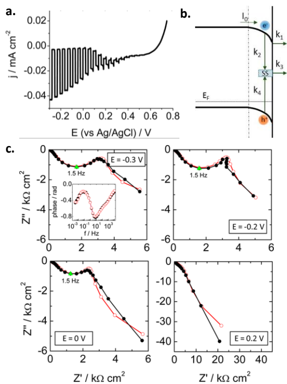
Fig. 10 (a) Linear sweep voltammogram under transient illumination for a calcium ferrite electrode. (b) Scheme illustrating the different charge transfer processes at the p -type semiconductor-electrolyte interface (SEI). (c) Nyquist plots under illumination for different potentials showing experimental points (black solid symbols) and simulated curves (red open symbols). Points corresponding to \omega_{\max} are marked in green. Inset: experimental and simulated Bode plots at -0.3 V. Illumination: 93 mW·cm -2 , AM 1.5G. Electrolyte: N 2 -purged 0.1 M Na 2 SO 4 . Reprinted with permission from Ref. 143. Copyright 2016 American Chemical Society.
