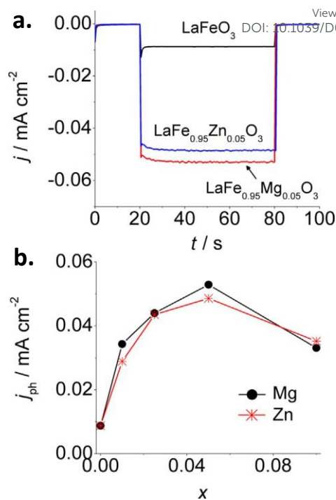
Fig. 9 (a) Photocurrent transients at -0.25 V vs Ag/AgCl for pristine \text{LaFeO}_3 and doped \text{LaFe}_{1-x}\text{M}_x\text{O}_3 ( \text{M} = \text{Mg} or \text{Zn} ) with x = 0.05 and (b) Stationary photocurrent at -0.25 V vs Ag/AgCl after 60 s of illumination as a function of x in \text{LaFe}_{1-x}\text{M}_x\text{O}_3 ( \text{M} = \text{Mg} or \text{Zn} ) electrodes in \text{O}_2 -purged 0.1 M NaOH. Reprinted with permission from Ref. 137. Copyright 2017 Wiley-VCH Verlag GmbH & Co.
