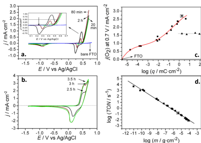
Fig. 6 (a, b) Cyclic voltammograms for bare FTO (blue line) and FTO/Ni(OH) 2 electrodes, corresponding to deposition times of (a) 20 min, 80 min and 2 h (green, red, and black lines, respectively) and (b) 2.5 h, 3 h and 3.5 h (black, red, and green lines, respectively). Inset: detail of the voltammetric curves in the high potential region. (c) Current density for the oxygen evolution reaction (OER) at 0.7 V for FTO/Ni(OH) 2 electrodes versus the charge density for the reduction of NiOOH. (d) Turnover number (TON) for the OER at 0.7 V for FTO/Ni(OH) 2 electrodes as a function of the Ni(OH) 2 deposited mass per unit geometric surface area. Reprinted with permission from Ref. 99. Copyright 2012 Hydrogen Energy Publications, LLC. Published by Elsevier Ltd.
