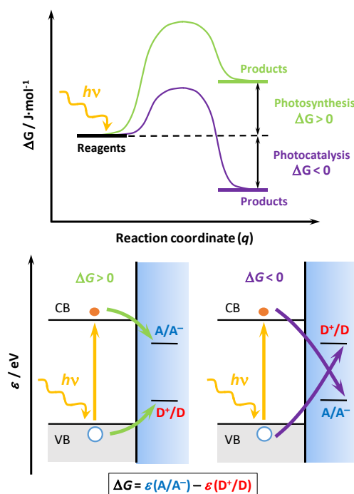
Fig. 1 Schemes for the energy vs. reaction coordinate curve (top) and the corresponding band structures (down) for two generic processes: photosynthetic (down left, green lines) and photocatalytic (down right, purple lines). Symbols: CB and VB, conduction and valence bands, respectively; A/A - , redox couple associated with the electron acceptor (A); D + /D, redox couple associated with the electron donor or hole acceptor (D); \Delta G , Gibbs energy of reaction; \epsilon , energy in the absolute scale; h\nu , photon energy; q , reaction coordinate. The equation below shows how to calculate \Delta G from the energies of each redox couple. Grey and blue shaded areas represent the filled VB states and the electrolyte, respectively. The top scheme was adapted from ref. 6, and the down scheme was adapted from Refs. 11 and 12.
