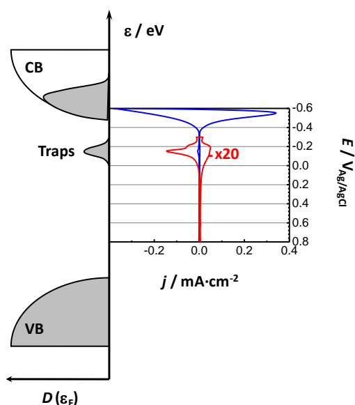
Fig. 3 Scheme of the correlation between the cyclic voltammogram obtained in the dark in the absence of faradaic currents and the electronic density of states (DOS) for a
