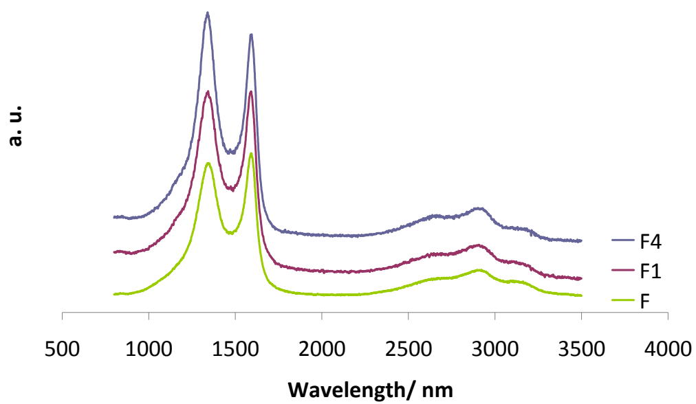
Figure S4. Raman spectra of the studied nanoporous carbons.
