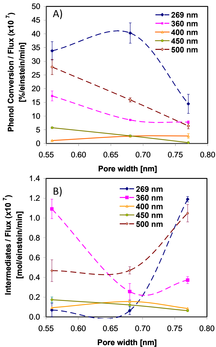
Figure 3. Correlation of normalized phenol photooxidation conversion (A) and intermediates detected (B) with the mean micropore size at different wavelengths.
