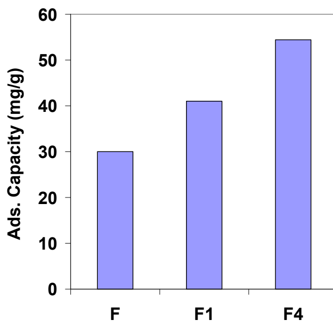
Figure S3. Limiting phenol adsorption capacity (mg/g) of the studied nanoporous carbons.
