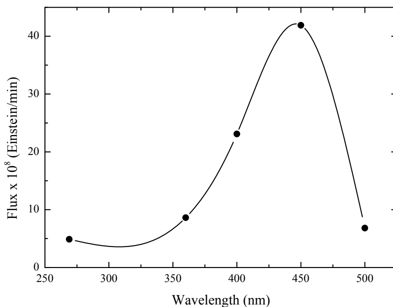
Figure S1. Photon flux at each individual wavelength for the irradiation set-up used coupled to monochromator.
