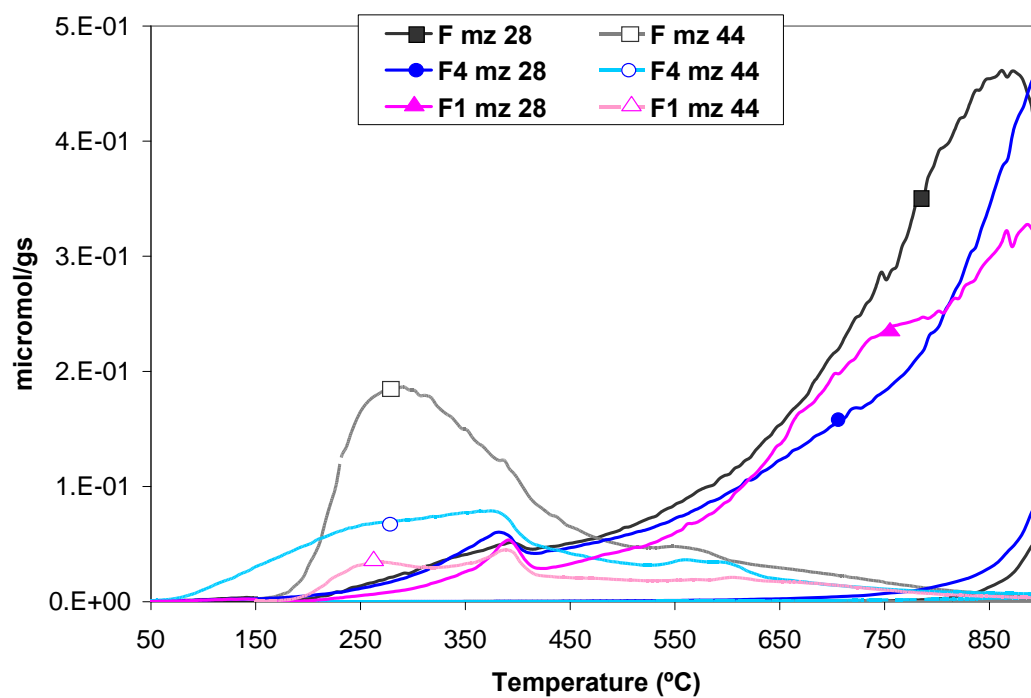
Figure S2. TPD-MS of the studied nanoporous carbons corresponding to the amount of CO and CO 2 evolved.
