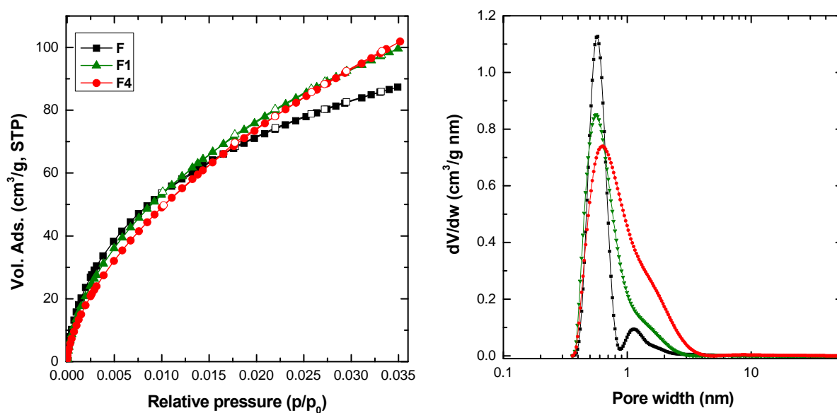
Figure 1. (left) Carbon dioxide adsorption isotherms measured at 0 °C showing the differences in the narrow microporosity of the studied carbons. (right) Pore size distributions obtained from the 2D-NLDFT-HS model applied to the N 2 adsorption isotherms at -196 °C.
