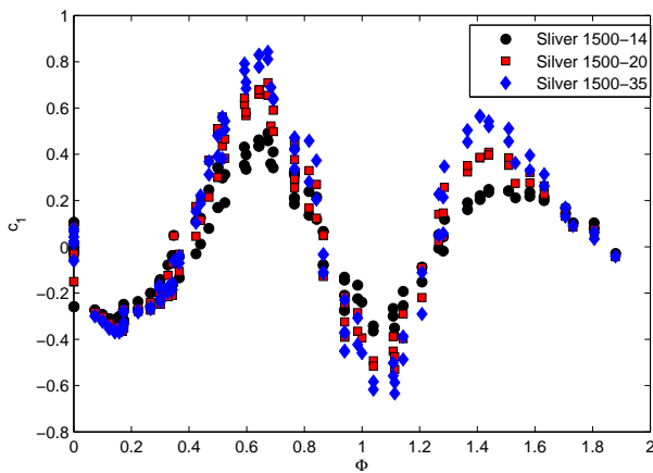
Fig. 12. Variation with \Phi of the first weighting coefficient, c_1 , of coatings Silver 1500-14, Silver 1500-20 and Silver 1500-35, having different diffraction pigment sizes (14 \mu\text{m} , 20 \mu\text{m} and 35 \mu\text{m} , respectively).
