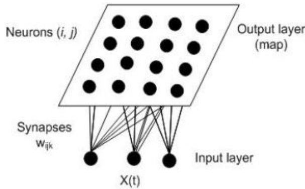
Figure 2: Structure network Self-Organizing Maps
