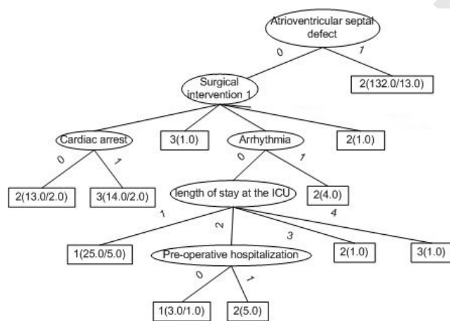
Figure 3: Part of the structure of our decision tree C4.5
