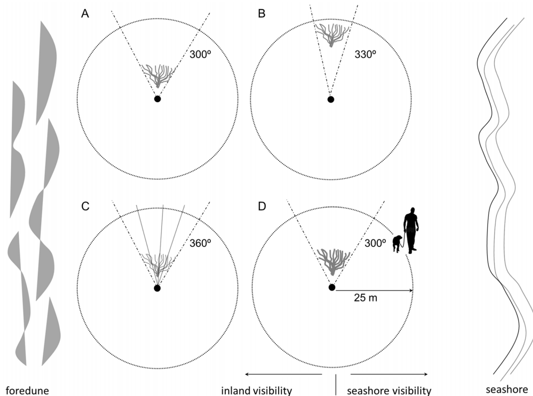
Figure 3. Experimental design to record visibility from Kentish Plovers' nests. Black dots show the location of Kentish plovers' nests. Circular dashed lines show the perimeter of the circle (25 m radius) in which the visibility of both humans and dogs were recorded. Inland and seashore visibility were recorded separately by dividing the circle in two 180^\circ sectors parallel to the seashore. The figure illustrates four different situations in which vegetation may obstruct plovers' view: a plant close to the nest (A) obstructs more ( 60^\circ of view occluded) than the same plant farther from the nest (B) ( 30^\circ of view occluded). In addition, a plant located at the same distance from the nest may allow the visibility through it (C) or may obstruct totally the visibility (D) depending on the permeability of the foliage density. doi:10.1371/journal.pone.0107121.g003
