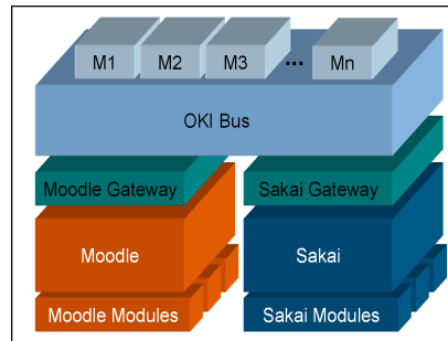
Fig. 1: Three-layered architecture using the OKI in the middleware
