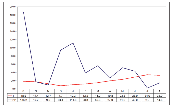
Fig. 4. Data for the hydrological year 2009–2010. PP: total monthly precipitation; T: medium monthly temperature. Total annual precipitation: 653 mm.
