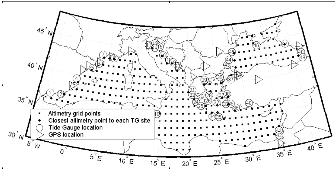
Figure 1. Data locations used in this study.
