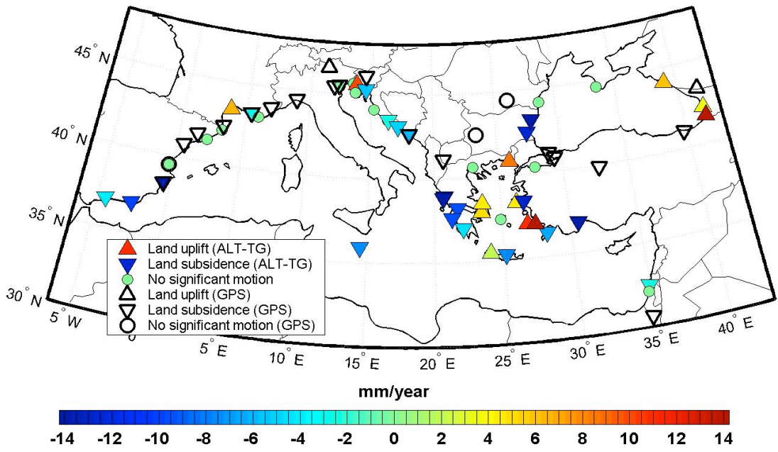
Figure 3. Vertical land movement along the Mediterranean and Black Sea coasts derived from Alt-TG time series.
