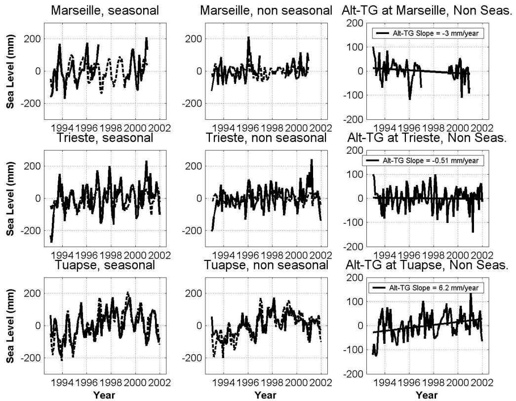
Figure 2. The first and second columns show seasonal and not seasonal Alt (solid line) and TG (dashed line) time series at Marseille (first row), Trieste (second row) and Tuapse (third row). The third column shows the non-seasonal Alt-TG time series and the least-squared linear fit to give the slope.
