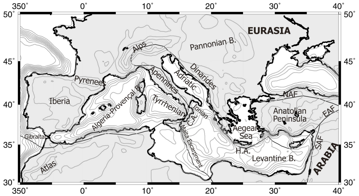
Figure 4. Black lines represent the plates boundaries in the Mediterranean and Black Seas from JIMENEZ-MUNT et al. (2003) (with permission from the author). H. A., Hellenic Arc; C. A. Calabrian Arc; B., Basin; NAF, North Anatolian Fault; SAF, South Anatolian Fault; EAF, East Anatolian Fault. Grey lines represent the topography of the region every 500 m. Note that the grey lines on the continents are positives and those on the sea are negatives, being zero on the coast line.
