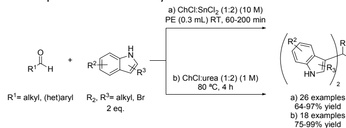
Scheme 3. Condensation of aldehydes and indoles.
