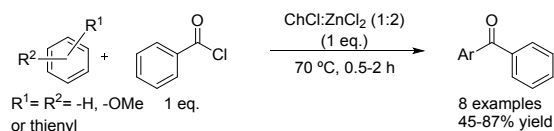
Scheme 17. Friedel-Crafts acylation of different arenes with benzoyl chloride using choline chloride: zinc chloride (1:2).
