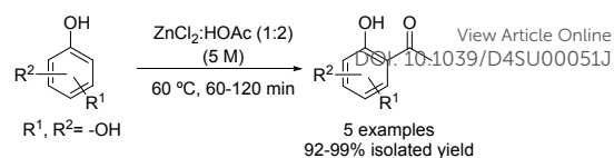
Scheme 19. Friedel-Crafts acylation of phenols using zinc chloride: acetic acid (1:2).
