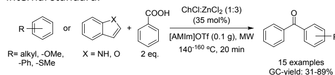
Scheme 15. Friedel-Crafts acylation of different arenes with carboxylic acids using a binary mixture formed by ChCl: ZnCl 2 (1:3) and [AMIm]OTf.
