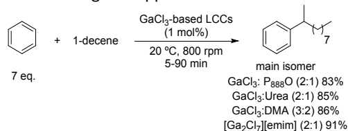
Scheme 5. Alkylation of benzene using 1-decene in GaCl 3 -based liquid coordination complexes.
