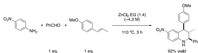
Scheme 13. Preparation of triarylmethane compounds using different DES.
