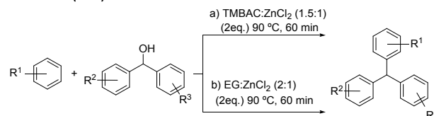
Scheme 12. Preparation of triarylmethane compounds using different DES.
