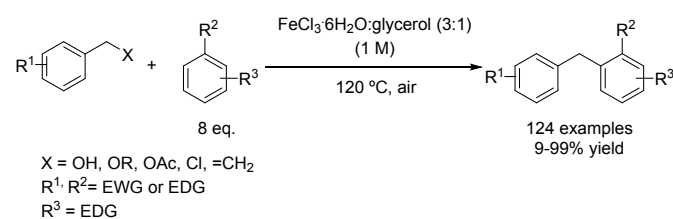
Scheme 6. FeCl 3 /glycerol promoted synthesis of diarylalkanes.
