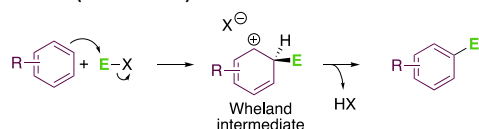
Scheme 1. General scheme of a S_E(\text{Ar}) reaction.
