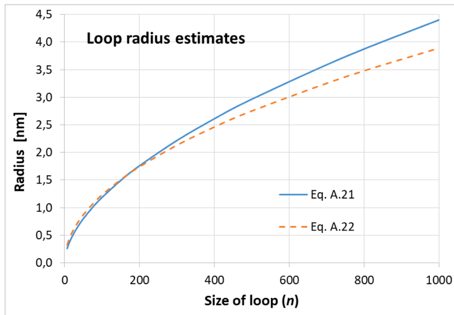
Fig. A.2. Estimates of the radius of a \frac{1}{2}\langle 111 \rangle loop according to the two approximations discussed in the text.
