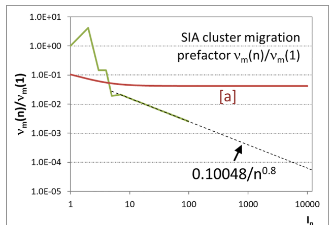
Fig. 8. Attempt frequency for SIA cluster migration \nu_m(n) , normalised over \nu_m(1) , versus cluster size as obtained from MD simulations [64] and function used to extrapolate to any size according to eq. (22), as well as to eq. (21), the latter denoted as [a].
