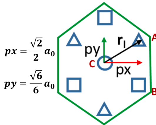
Fig. A1. The smallest perfect \frac{1}{2}\langle 111 \rangle loop (7 SIA) represented on the \{111\} crystallographic plane, formed by SIA located on three atomic planes, indicated by different geometrical figures. The distances indicated on the figure are used in the text to calculate the radius of the loop.
