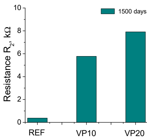
Figure 8. Resistance R_2 results noted for the mortars tested.
